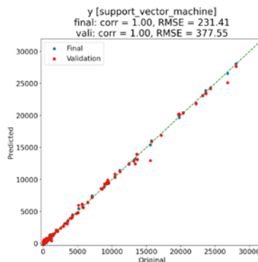
fig. 2: Optimized Hyperparameter
